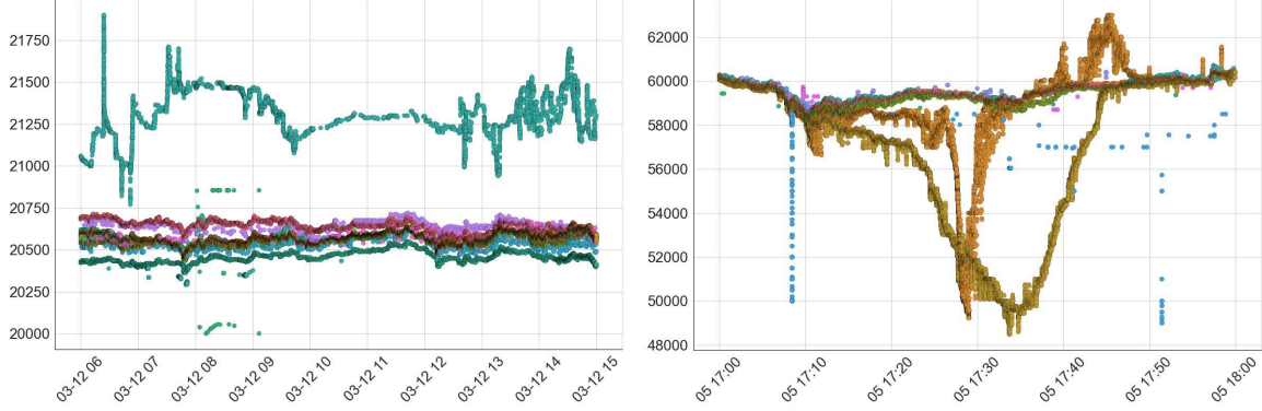
Figure 4: Illustrations of how Centralized Exchanges (CEXes) prices may differ. Each color corresponds to a different CEX. On the left-hand side, trade prices of the BTC-USD rate on March 12, 2023 between 6:00AM and 3:00PM UTC. On the right-hand side, trade prices of the BTC-EUR rate on March 5, 2024 between 5:00PM and 6:00PM UTC. Source: https://www.kaiko.com/products/data-feeds
