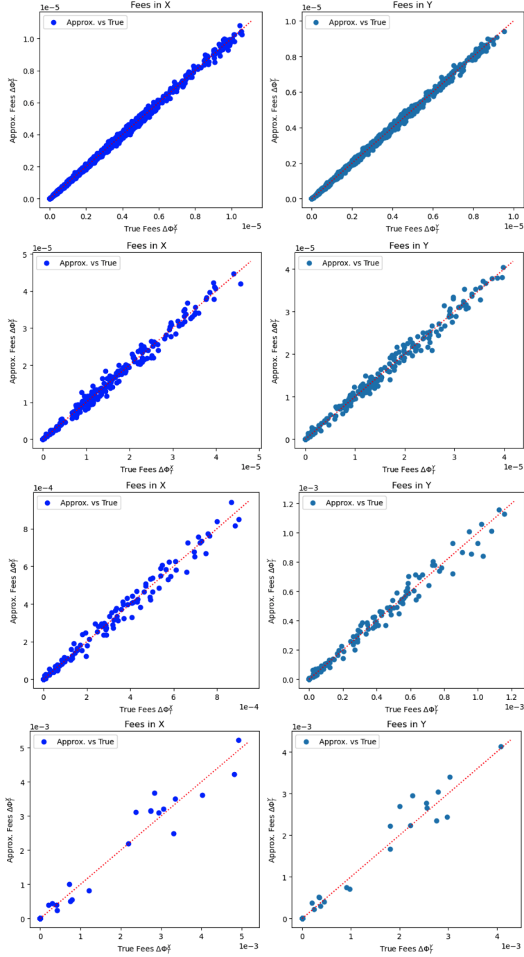
Figure 9: True collected fees versus their approximations. From top to bottom: \phi = 0.01\%, 0.05\%, 0.3\%, 1\% (related to \delta_\pi = 2, 10, 60, 200 ), T = 1/12, 1/12, 1, 1 . Each point corresponds to the amount of swap fee on a range; smaller values of \delta_\pi have more ranges hence more points.
