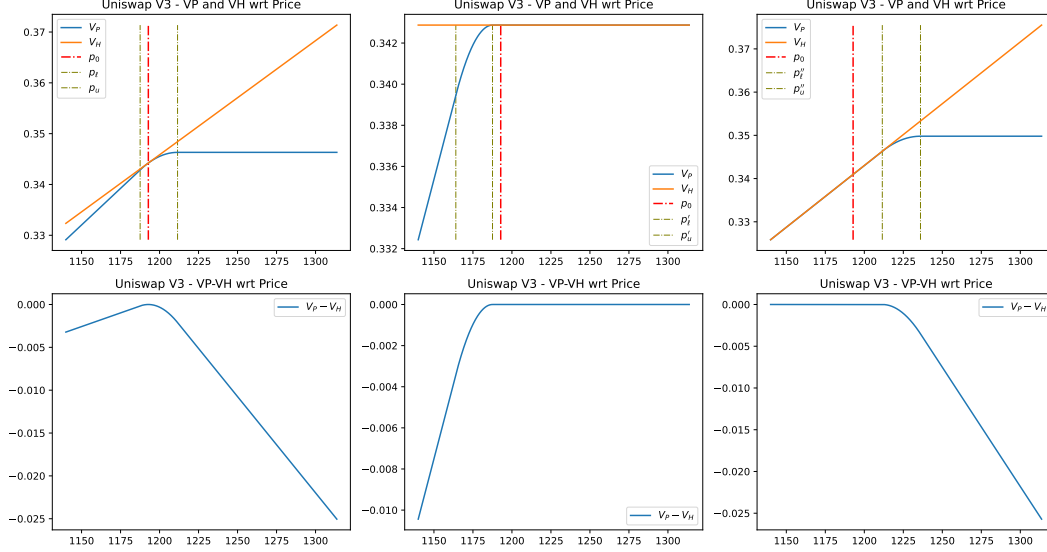
Figure 5: Values at time t_1 of V_P , V_H (top) and V_P - V_H (bottom) for 3 different price ranges. The x -axis corresponds to the price value p_1 at time t_1 . The dashed vertical lines in olive color represent the considered unitary ranges. At the initial price p_0 , the values V_P and V_H coincide.
