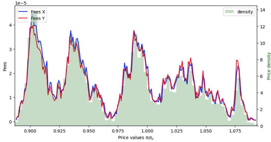
Figure 8: Left axis: the exact fees collected in tokens \mathcal{X} and \mathcal{Y} . Right axis: occupation density of p . Here, \delta_\pi = 10 , \phi = \gamma = 0.05\% , T = 1 month.
