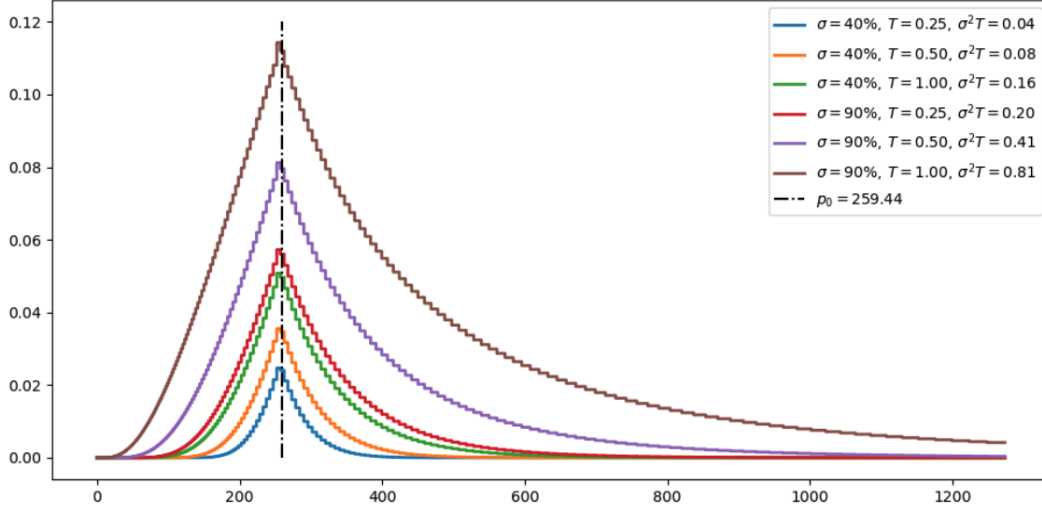
Figure 10: In the Black-Scholes model, representation of the expected fees (Equation (41)) as a function of square root price ranges, for different volatilities ( \sigma = 40\%, 90\% ) and different time horizons ( T = 0.25, 0.5, 1 ), with \delta_\pi = 200 , \phi = \gamma = 1\% .
