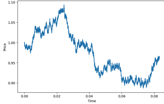
Figure 7: Sample path of p , with p_0 = 1 , \sigma = 40\% and drift \mu = 5\%
